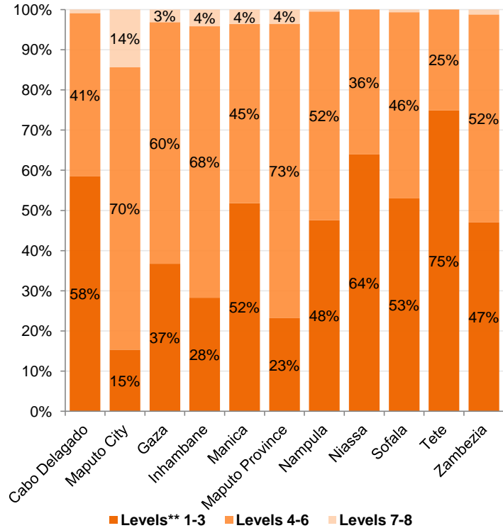
Performance on the reading assessment by region
